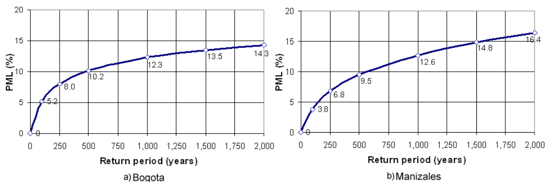
Figure 5. LEC results for several return periods for buildings in two cities of Colombia
