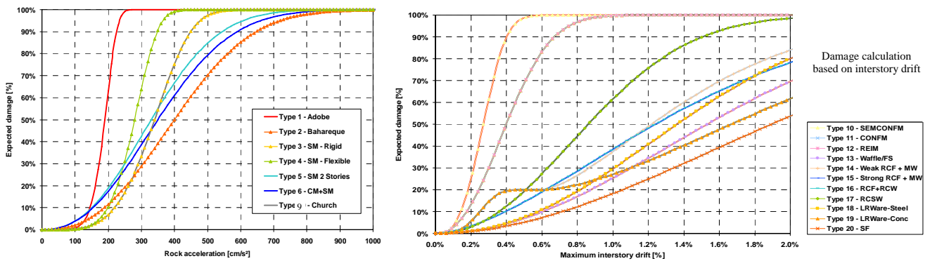
Figure 4. Vulnerability curves used for different construction classes in Colombia. a) Damage calculation based on acceleration. b) Damage calculation based on interstory drift
