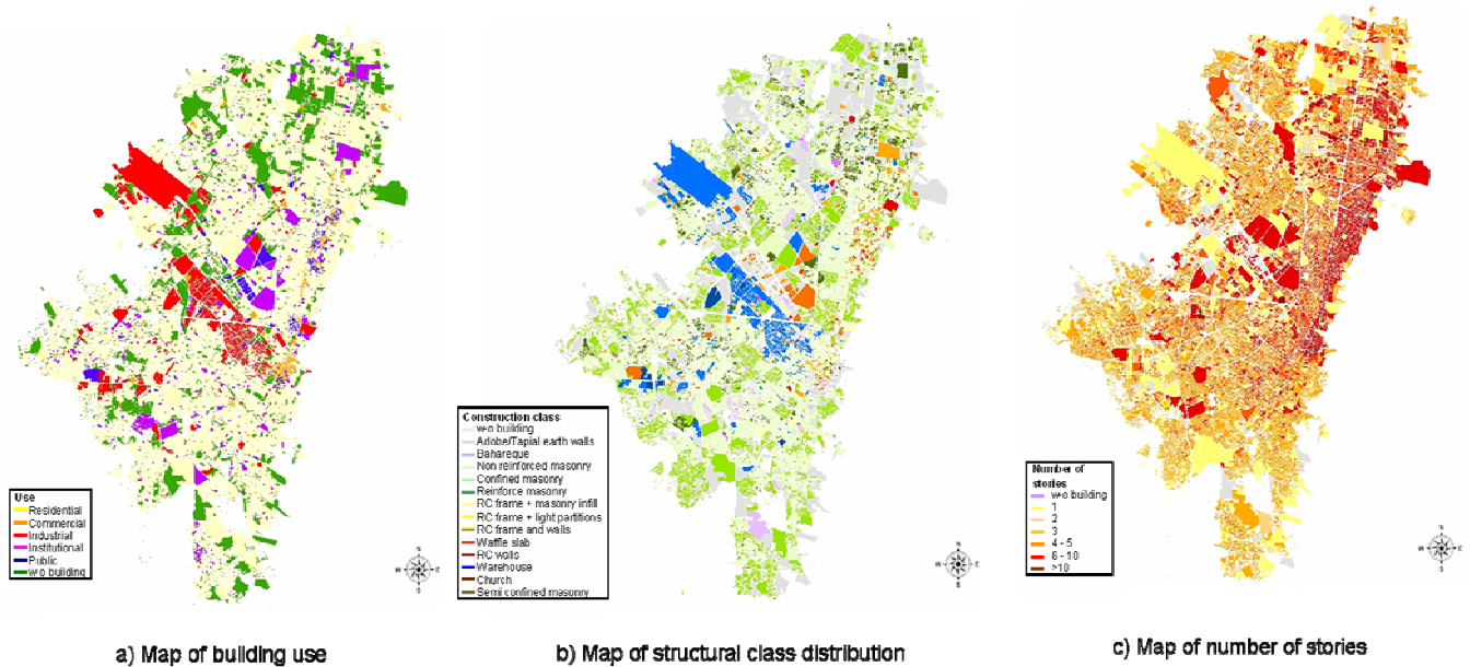
Figure 3. Index maps of a) building use, b) structural class distribution and c) number of stories for Bogotá
