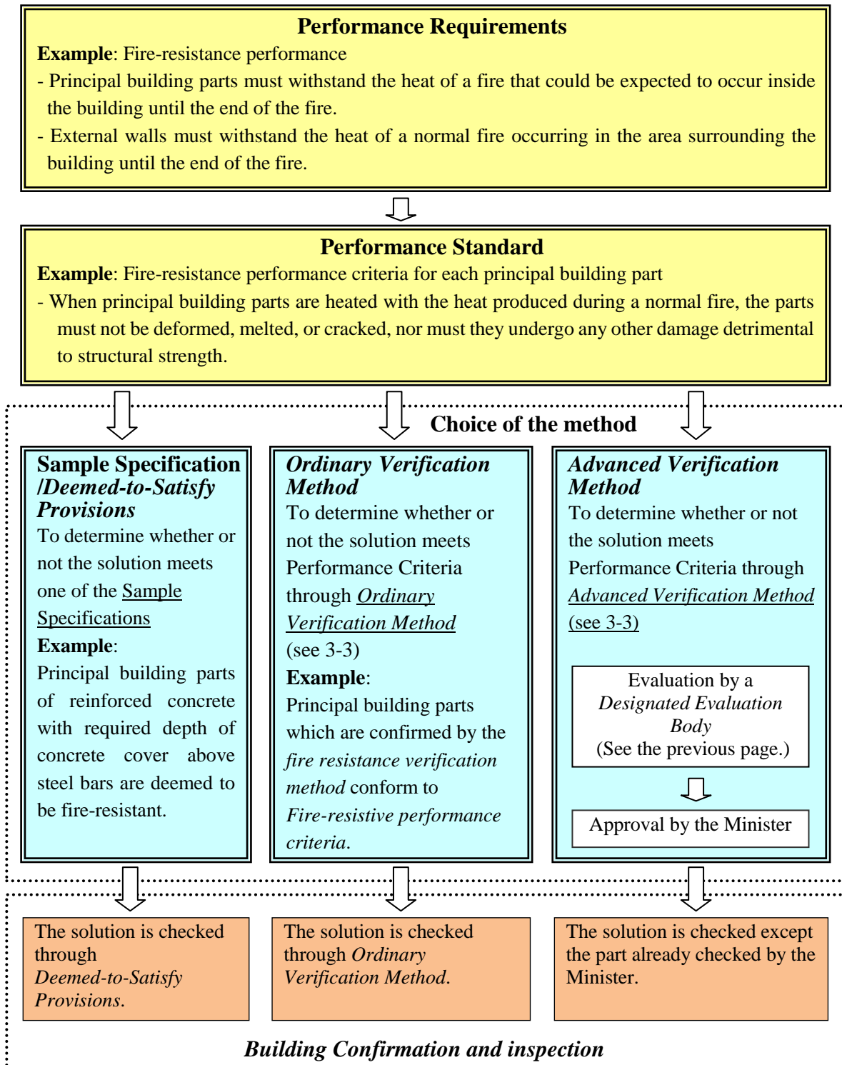
Figure 5 Structure of Performance-based Codes
