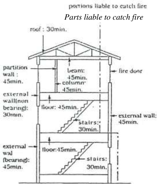
Figure 10 Quasi fire-resistive building
