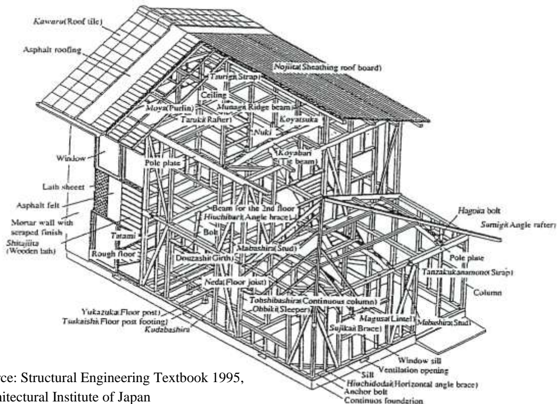
Figure 7 Structure of Traditional Japanese Wooden Houses
