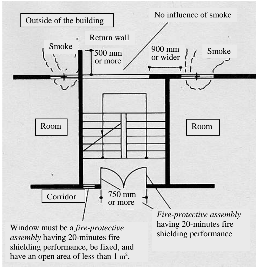
Figure 12 Escape Stairs (Example)
