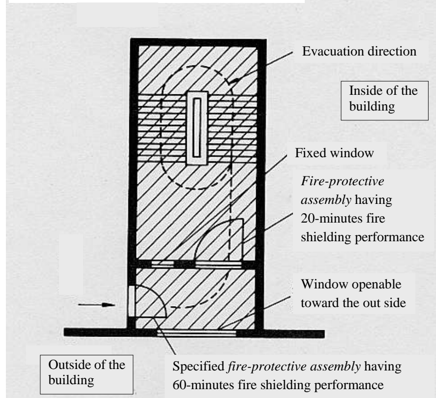
Figure 13 Special Escape Stairs (Example)
